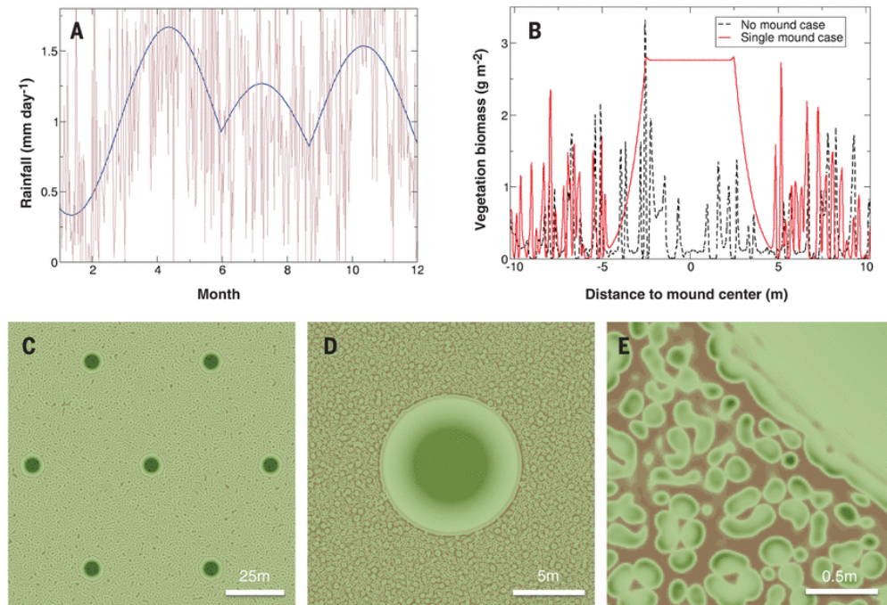
Fig. 2. Vegetation patterns obtained with stochastic rainfall and termite-induced heterogeneity. (A) Stochastic rainfall (brown curve) based on observed mean-monthly rainfall (blue curve) at MRC, 1999–2013. (B) Transect of predicted vegetation biomass density through a mound (solid curve) and in the absence of mounds (dashed curve). (C to E) Model outputs showing (C) 123-by-123-m region encompassing seven hexag-
