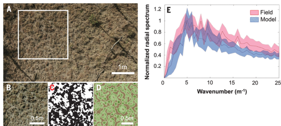
Fig. 3. Correspondence of predicted and observed vegetation patterns. (A) Photograph of 3.5-by-6-m region of matrix vegetation taken from 10 m height. (B) 1.5-by-1.5-m section used in the analysis, from white square in (A). (C) Binary transformation of (B) (white represents vegetation, black represents soil). (D) Model output used for comparison, with parameterization as in Fig. 2. (E) Normalized radial spectrum of real images ( n = 14 samples) and model simulations ( n = 192 samples), as a function of wave number.
