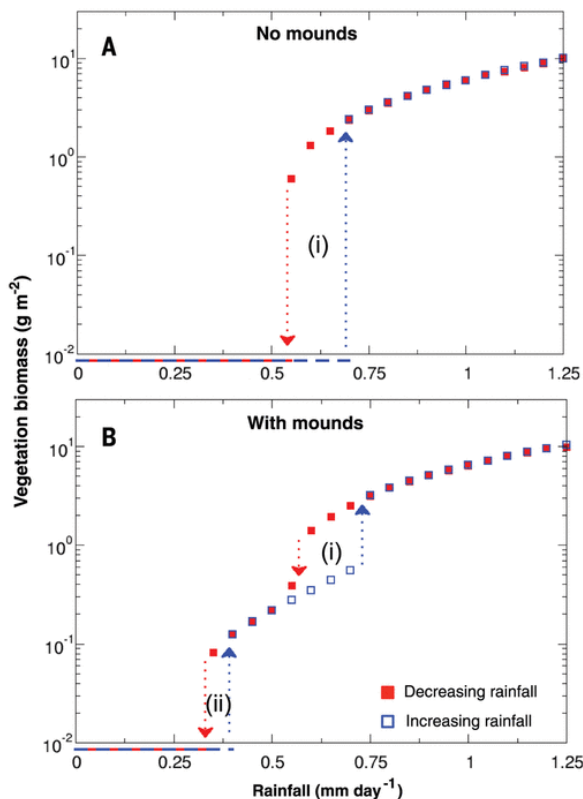
Fig. 4. Termite mounds increase ecosystem robustness. (A and B) Semilogarithmic phase diagrams under increasing (blue) and decreasing (red) rainfall for (A) model with no termite mounds and (B) the modified model with 50% on- versus off-mound improvement in both growth rate and infiltration efficiency. (A) Without mounds, one hysteresis cycle occurs (i), corresponding to sudden transitions to and from desertification. (B) Adding mounds generates two hysteresis cycles, corresponding to loss/recovery of matrix vegetation (i) and desertification/revegetation (ii). For both (A) and (B), we used fixed rainfall rates and parameters as described in table S1 and fig. S5.
